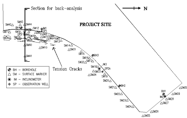
Fig. 4 Subsurface investigation and instrumentation layout
