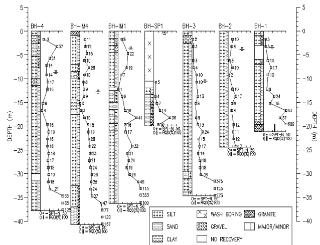
Fig. 5 Borehole logging
