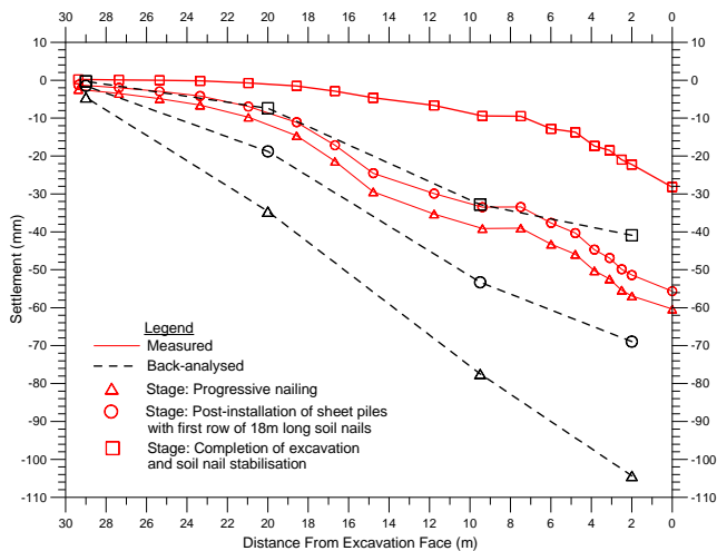
Fig. 9 Comparison of settlement on retained ground
