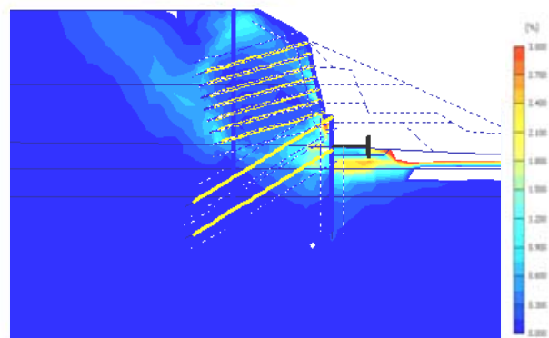
Fig. 11 Soil shear strain within the soil nail reinforcing system
