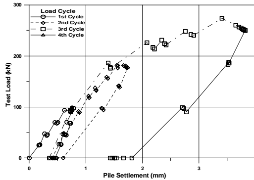
Figure 8 Working test pile (TP-2)
