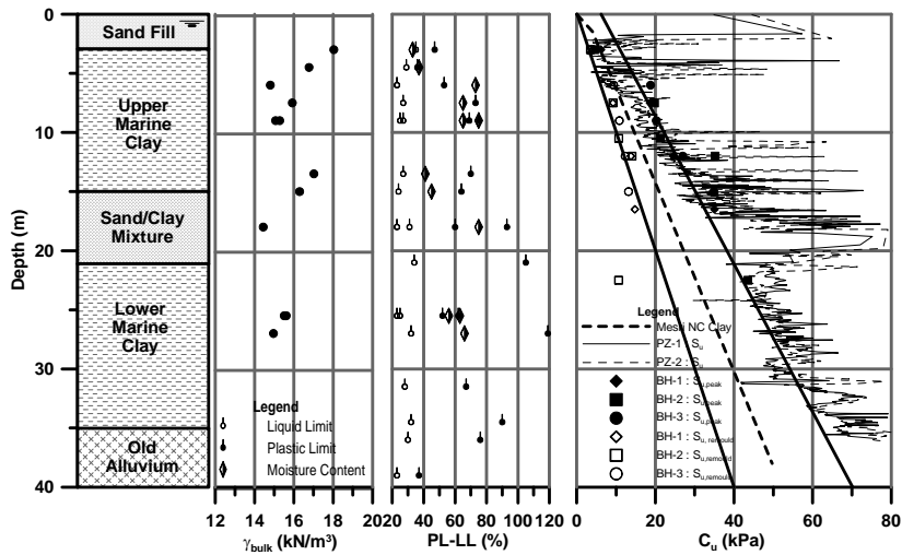
Figure 5. Interpreted subsurface condition.
