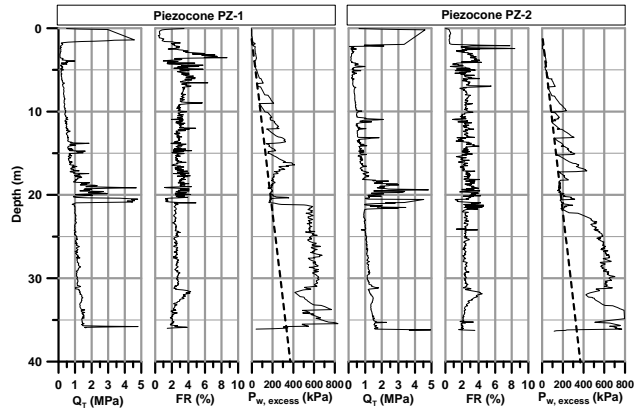
Figure 4. Piezocone results.
