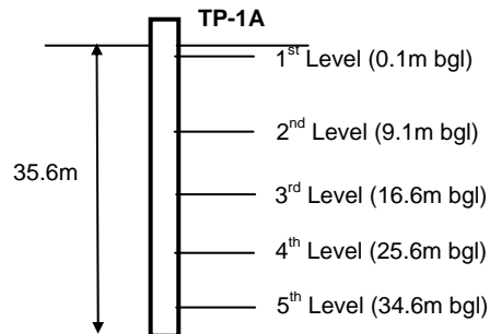
Figure 6. Location of strain gauges at TP-1A.
