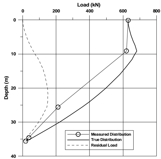
Figure 12. Residual and true load distributions.
