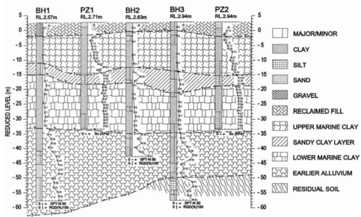
Figure 3. Subsurface profile of project site.
