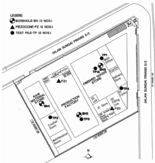
Figure 1. Project site layout plan.
