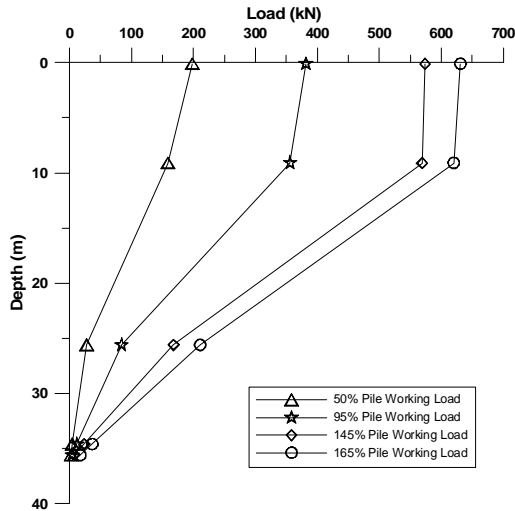
Figure 11. Measured load distribution (TP-1A).
