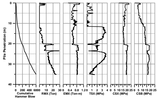
Figure 14. Driving monitoring results (TP-1A).
