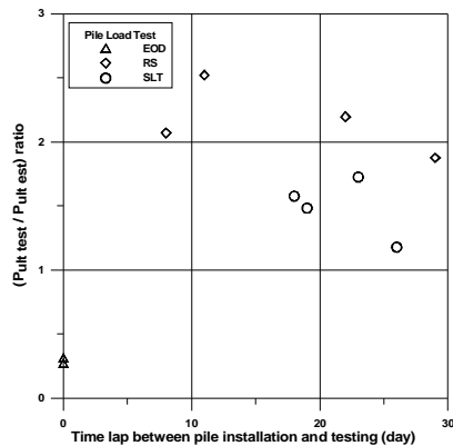
Figure 15. Development of pile capacity.
