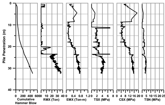
Figure 13. Driving monitoring results (TP-1).
