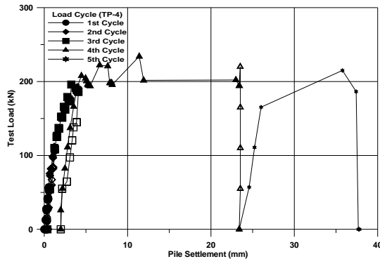
Figure 10 Working test pile (TP-4)
